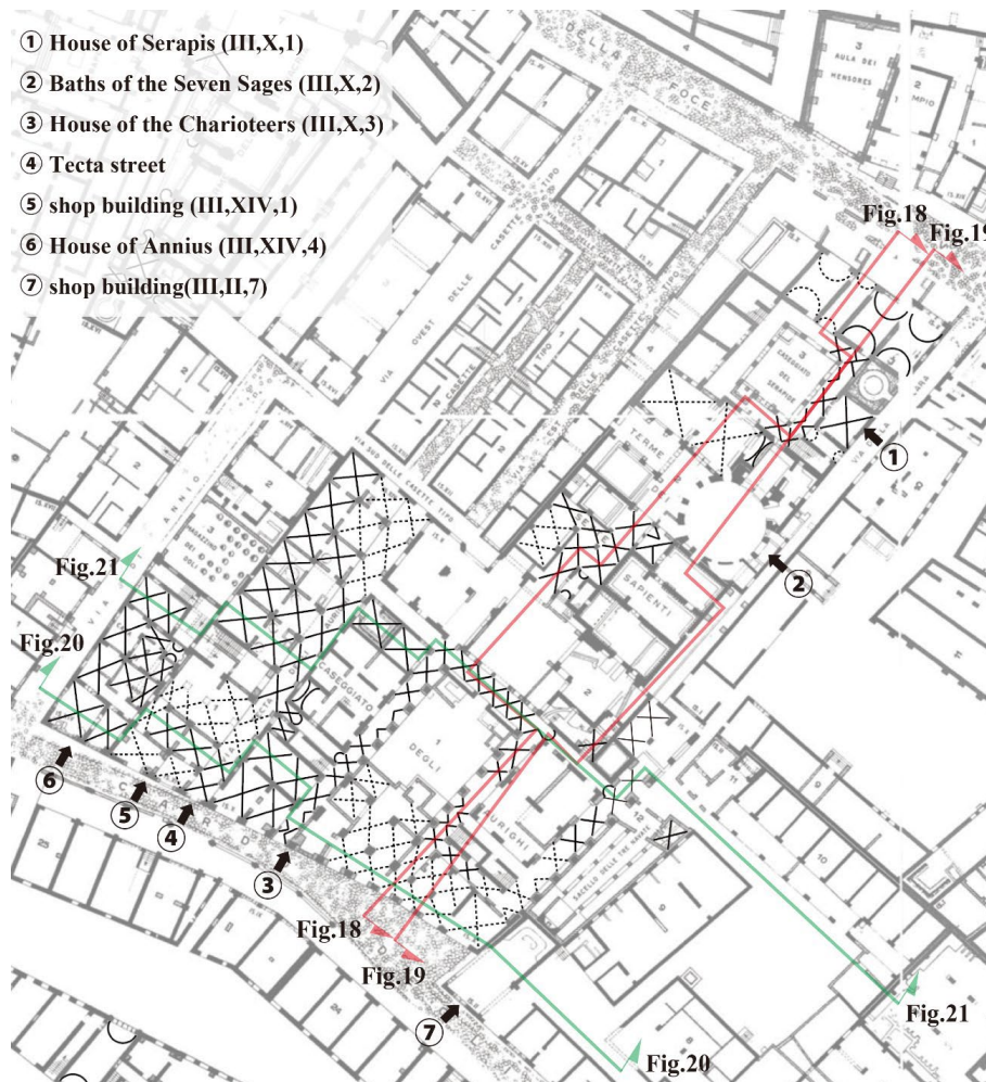
Figure 17. Clusters of Cross Vaulted Structures
