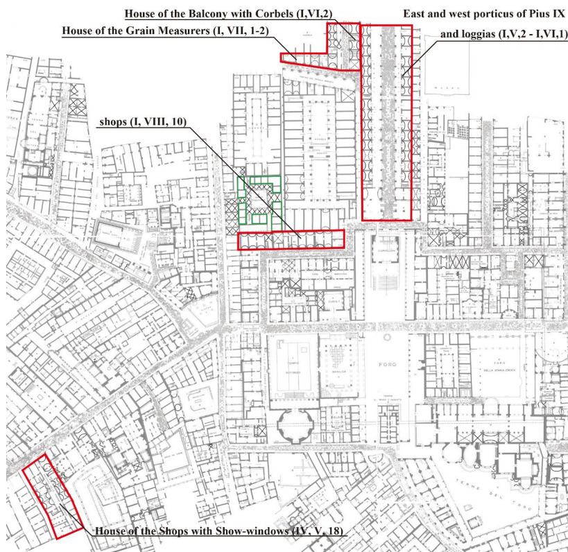
Figure 16. Clusters of Barrel Vaulted Structures
