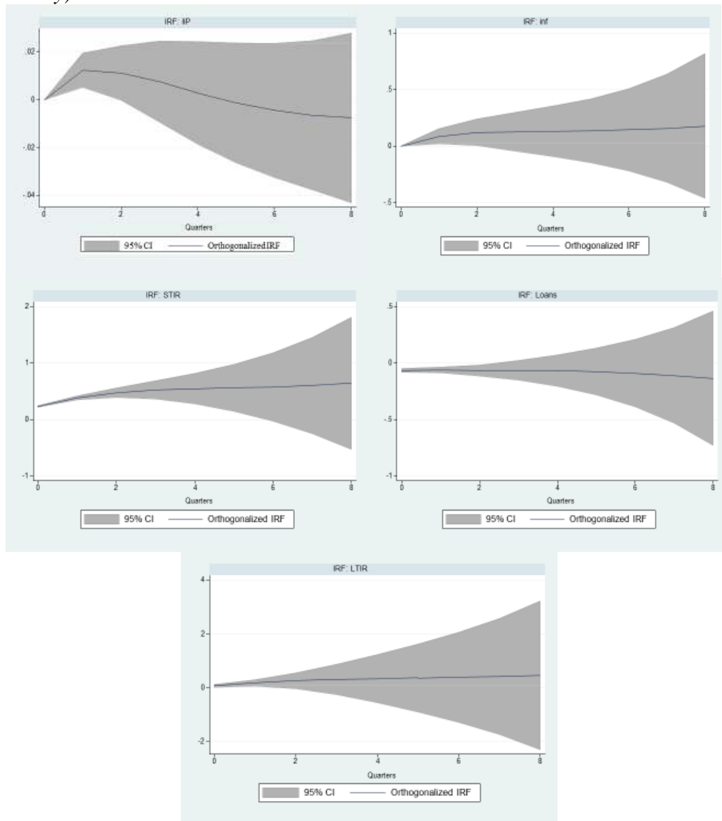
Figure 1. Impulse Responses of Variables to a One-Unit Shock in STIR (Monetary Policy)
