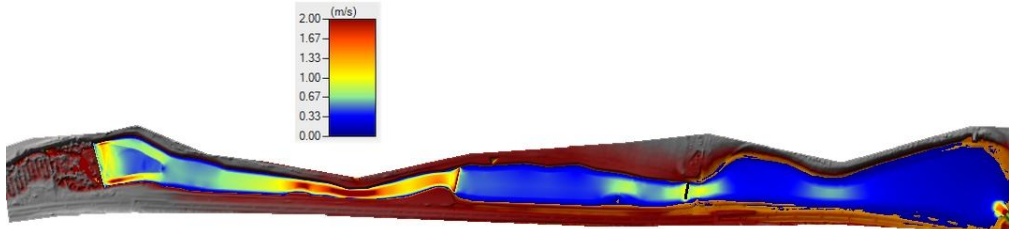
Figure 8. Maximum Velocities in the Lakes under High-flow Flood Conditions
