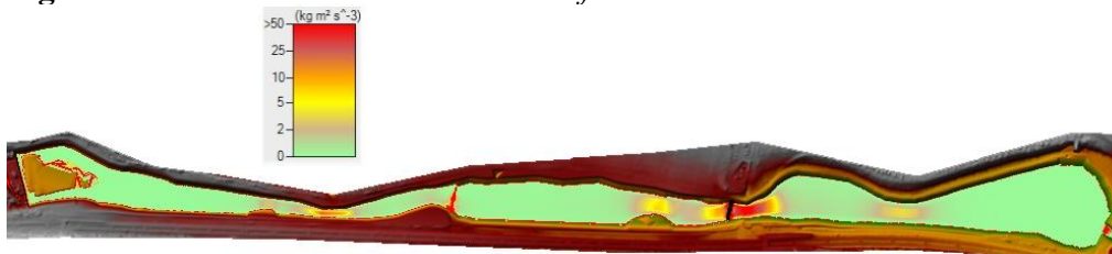
Figure 10. Stream Power Under Medium-flow Conditions
