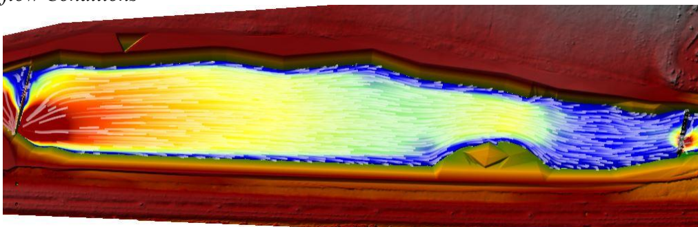
Figure 6. Flow Directions and Relative Velocities in the Middle Lake under Low-flow Conditions
