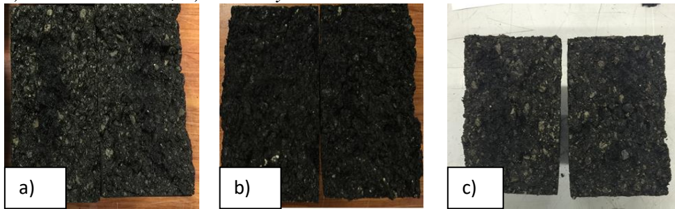
Figure 3. Investigation of Stripping of Wet Subset Samples after Testing. a) HMA; b) WMA-Evotherm; c) WMA-Sylvaroad
