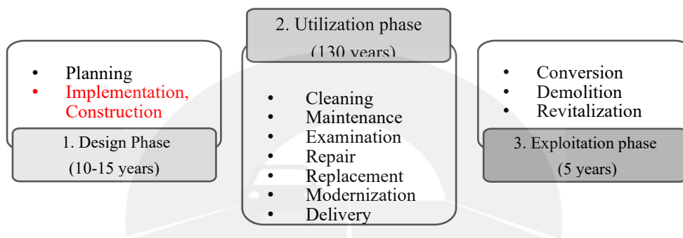
Figure 1. Phases and Processes in the Life Cycle of a Tunnel Structure
